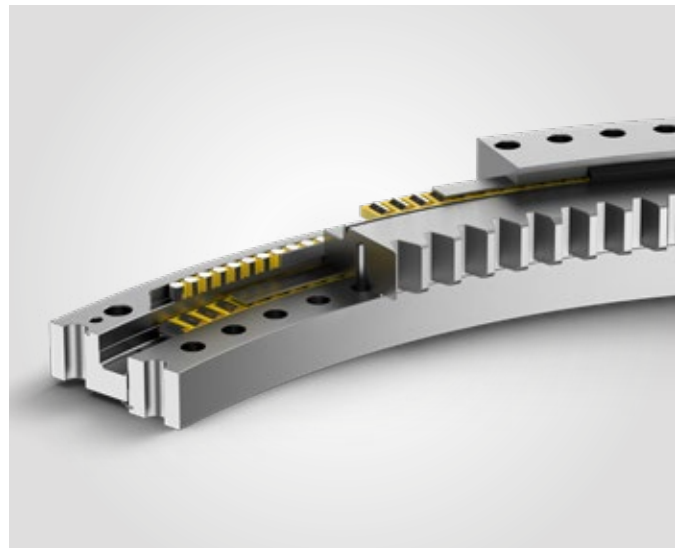
Through-hardened insert plates as raceway (optional)
