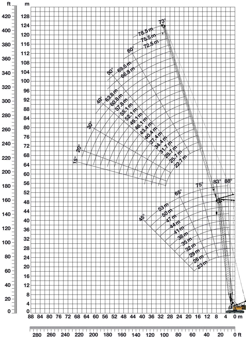
Boom configuration for main boom lengths (23 m - 53 m) (see table 1 on page 10) Jib configuration for jib lengths (22.7 m - 78.5 m)
