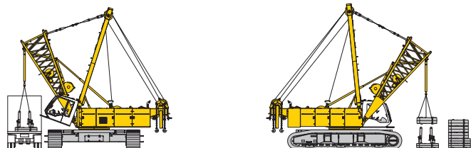
Unloading and assembly of counterweight
