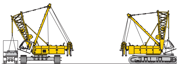
Unloading and assembly of carbody counterweight
